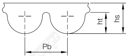
HTD圆弧齿Arc tooth
