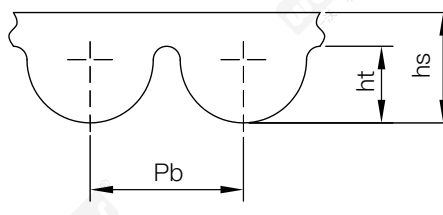
GT/YU齿同步带GT/YU tooth
