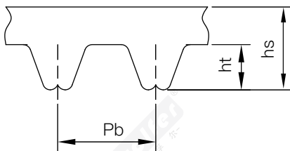
RPP/RHP圆弧齿Arc tooth
