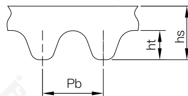
STPD/STS圆弧齿Arc tooth
