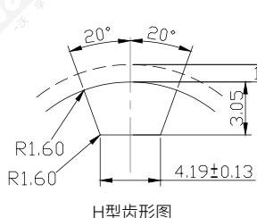
H型齿形图: Tooth form diagram
