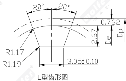
L型齿形图: Tooth form diagram
