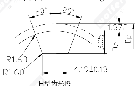
H型齿形图: Tooth form diagram
