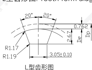
L型齿形图: Tooth form diagram
