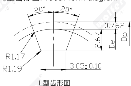
L型齿形图: Tooth form diagram
