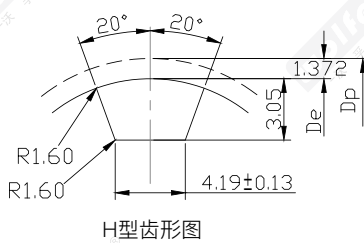
H型齿形图: Tooth form diagram
