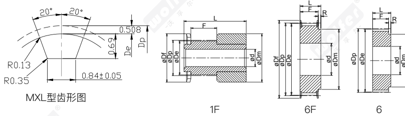
MXL型齿形图: Tooth form diagram
