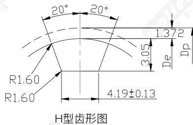
H型齿形图: Tooth form diagram
