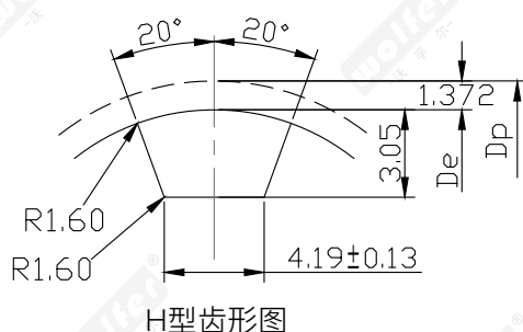
H型齿形图: Tooth form diagram
