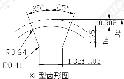
XL型齿形图: Tooth form diagram
