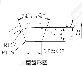
L型齿形图: Tooth form diagram
