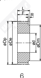
AT5型齿形图: Tooth form diagram
